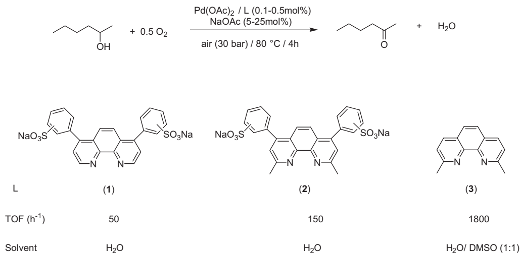
Figure 1. Palladium(II) complexes of dinitrogen ligands.
