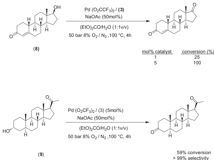
Figure 4. Aerobic oxidation of nandrolone ( 8 ) and 5α-pregnan-3α-ol-20-one ( 9 ).
