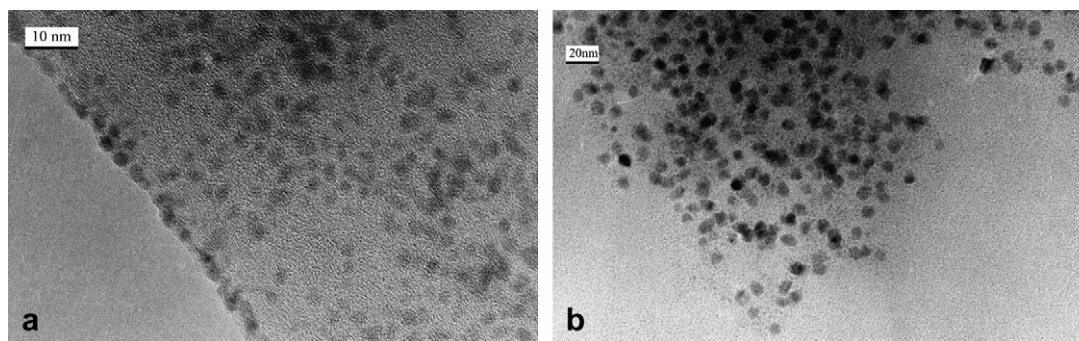
Figure 3. TEM photograph of Pd nanoparticles (a) before and (b) after oxidation reaction.
